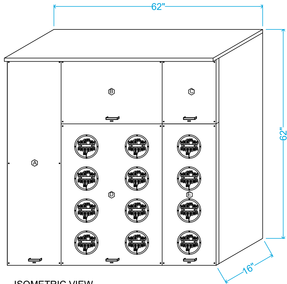
ISOMETRIC VIEW
